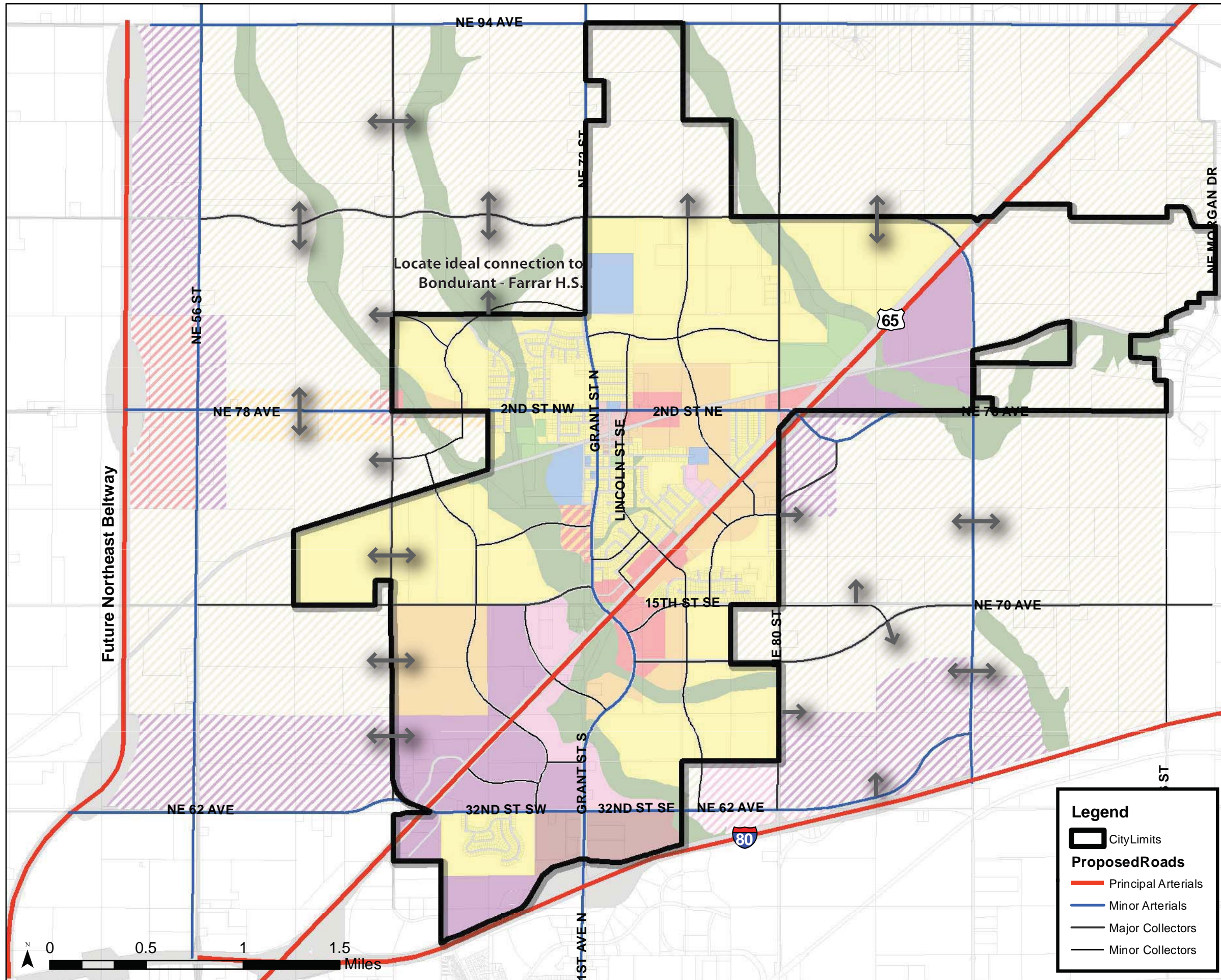
Figure 6.4 - Roadways Network
