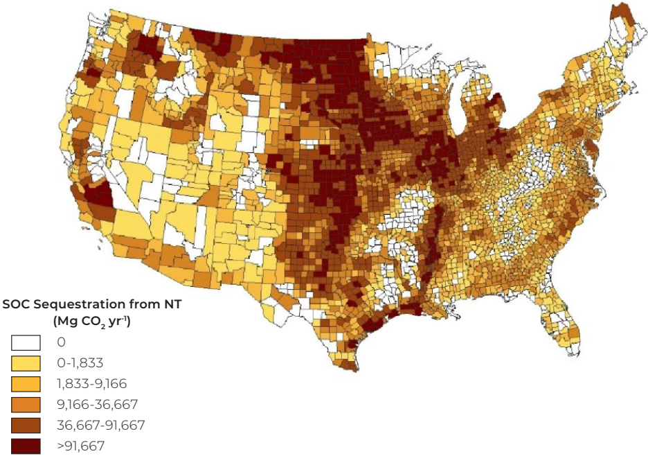
FIGURE 1 Sequestration Potential Map Source: Carbon Balance and Management Journal, Biomed Central. [7]
